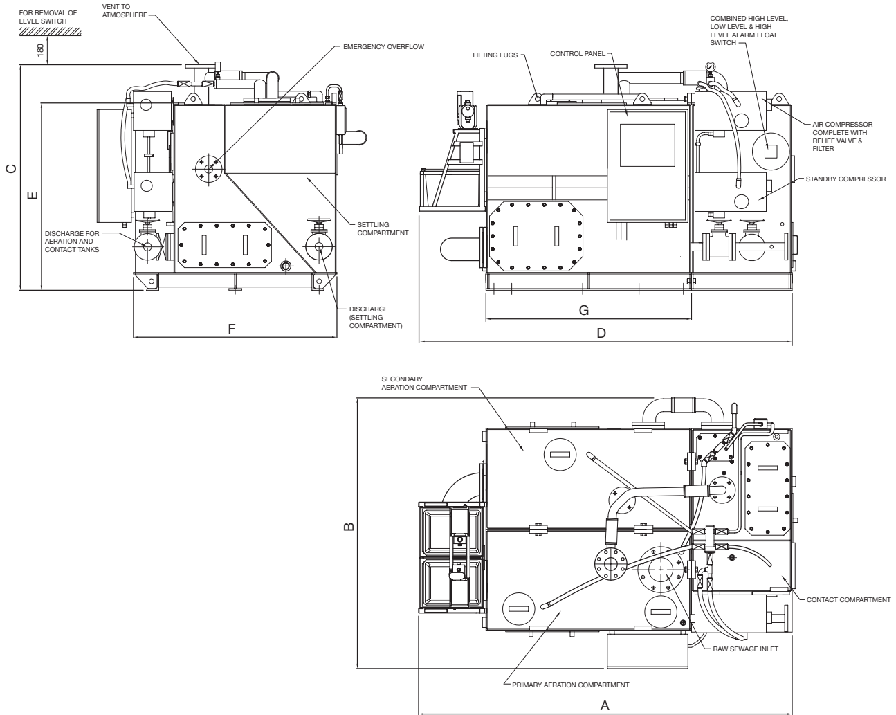
Fig.1 Detailed elevation drawings
