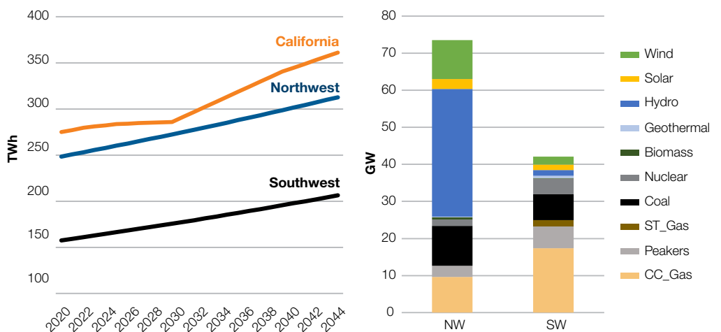
Figure A2-1. Electricity demand by regions (left) and Initial Installed capacity in NW and SW Regions (right).
