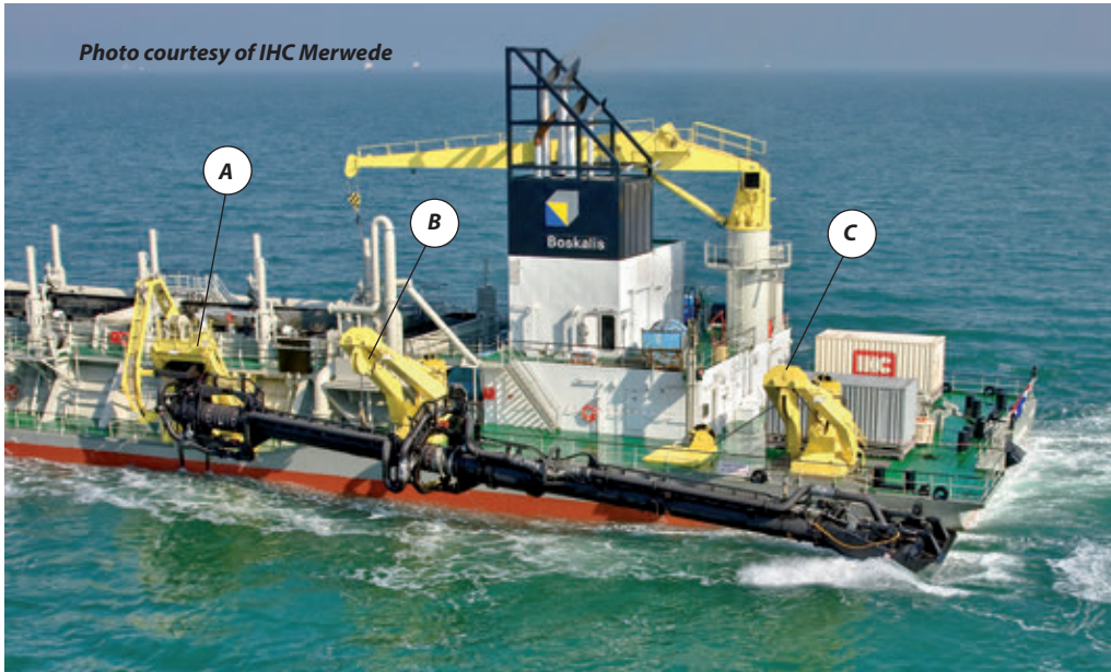
Gantries and drag arm A – Trunnion gantry, B – Intermediate gantry, C – Draghead gantry
