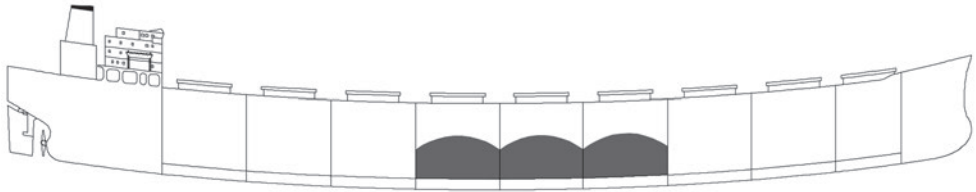
Sagging in still water created by the wrong cargo loading
