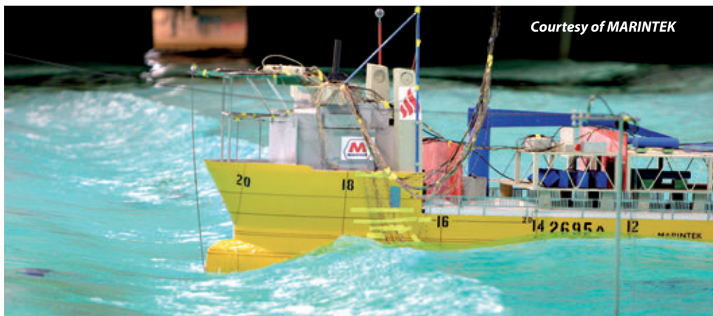
Seakeeping test
