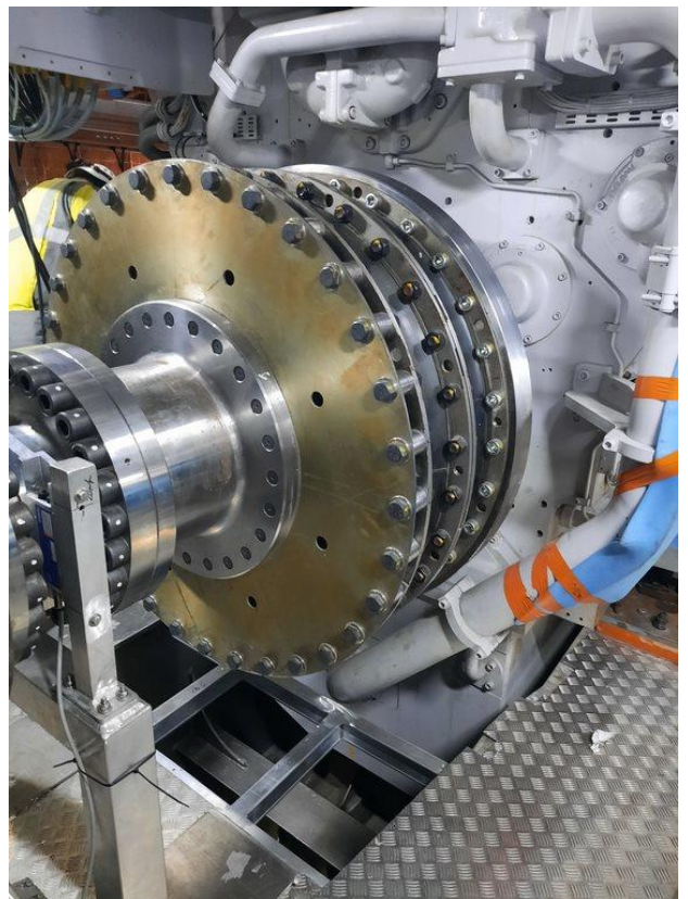
Image 6: Coupling between main engine and gearbox
