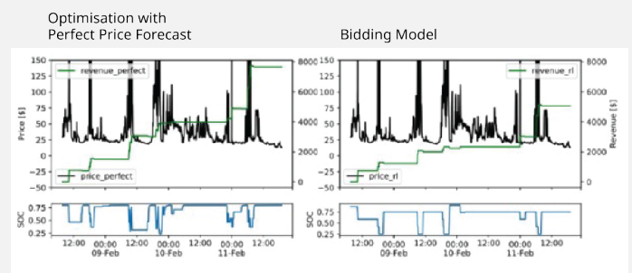
Figure 2: Example of three-day comparison of GEMS IntelliBidder bid optimisation to a perfect forecast benchmark.
