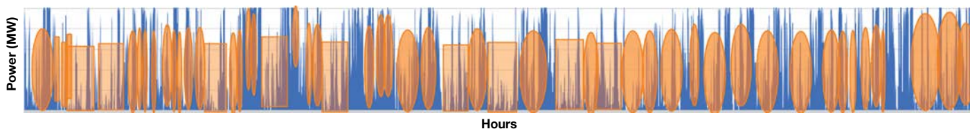
An illustrative example of annual wind generation from Southeast Asia (MW). The wind can be 100% generation and reduce to zero within 20 minutes.
