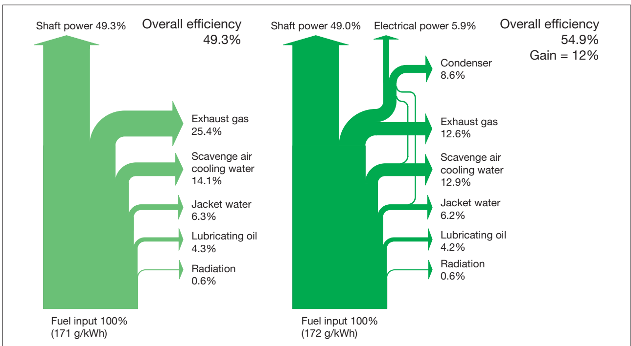
Fig. 12: Comparison of heat balances for Sulzer 12RT-flex96C engines without heat recovery (left) and with the Total Heat Recovery Plant (right) showing the 12% gain in overall efficiency for the Total Heat Recovery Plant. [04#048]
