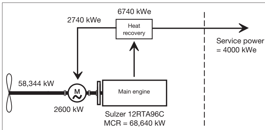
Fig. 14: Schematic of the propulsion system with the Total Heat Recovery Plant. [04#050]
