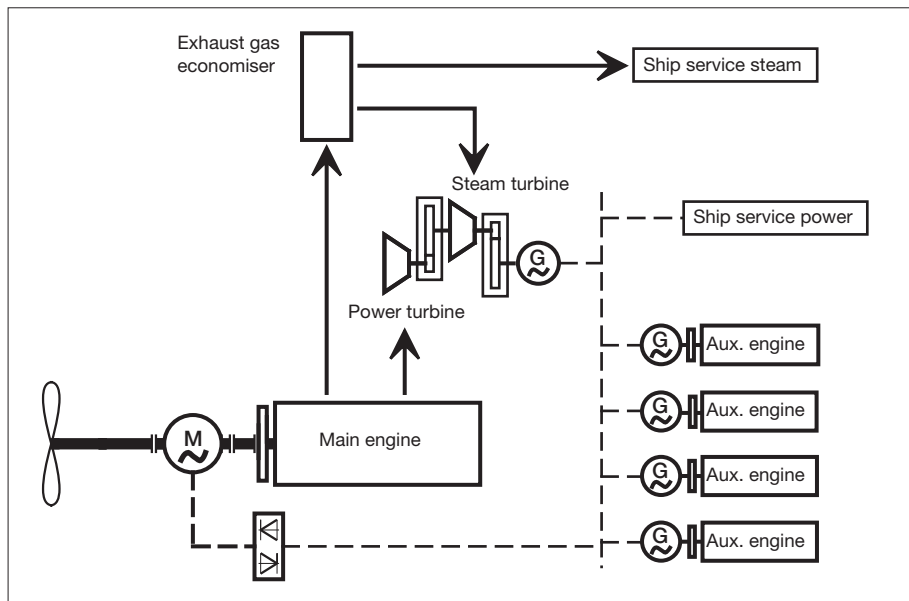
Fig. 4: Schematic of the Total Heat Recovery Plant. [04#040]
