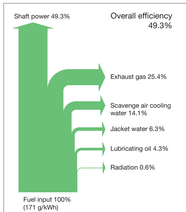
Fig. 1: Heat balance of a Sulzer 12RTA96C engine shows the potential for waste heat recovery with current large, low-speed marine engines. [04#037]
