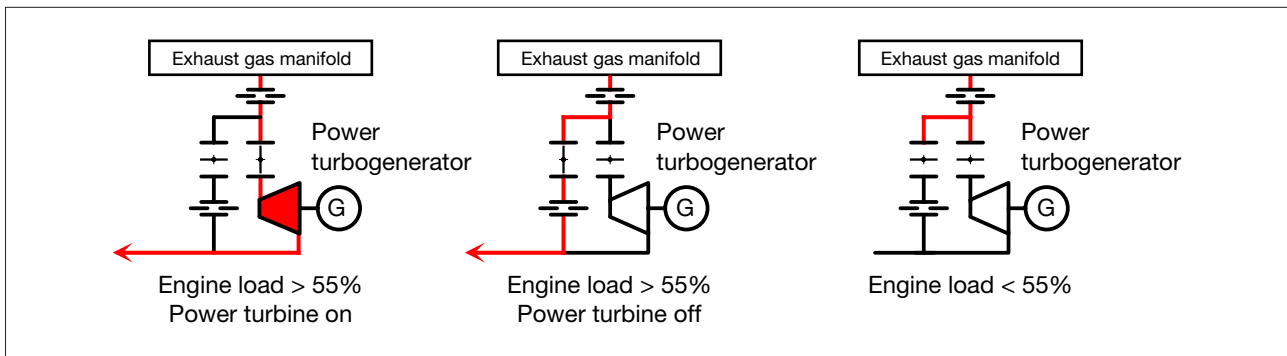
Fig. 7: Operating modes for the exhaust gas power turbine. [04#043]
