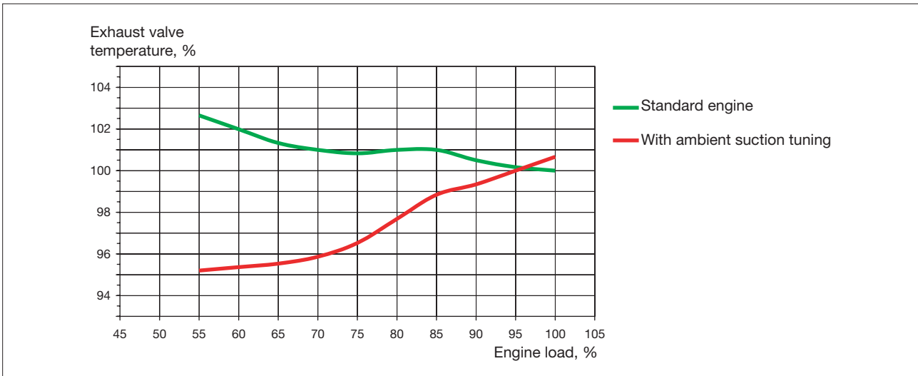
Fig. 3: Thermal loading of the engine with conventional tuning compared with that obtained when tuned for the Total Heat Recovery Plant as represented by the exhaust valve temperature for the 12RT-flex96C engine. [04#039]
