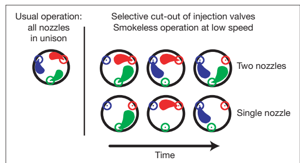
Fig. 17: Sulzer RT-flex engines are unique in that individual fuel injectors can be cut out as required. At most engine speeds the engines operate on all fuel injectors acting in unison in each cylinder. As speed is reduced, at first one injection valve is shut off and then at very low load speeds another injection valve is shut off leaving the engine running on all cylinders but with just one injector in operation in each cylinder. [03#118]
