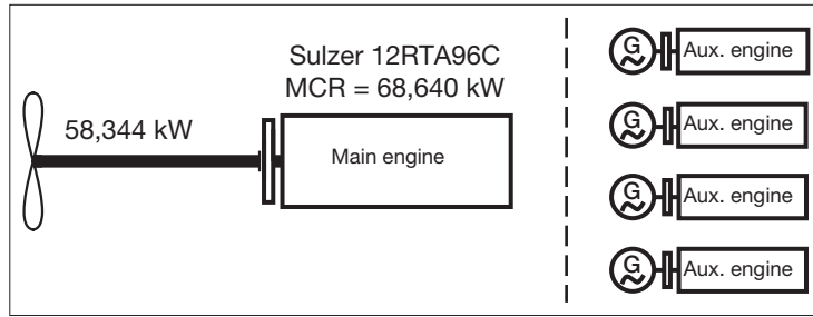
Fig. 13: Schematic of the conventional propulsion plant – the basis. [04#049]
