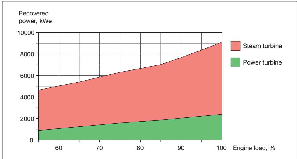
Fig. 11: Recovered power from a Sulzer 12RT-flex96C engine, average aged, average ISO/tropical conditions. [04#047]
