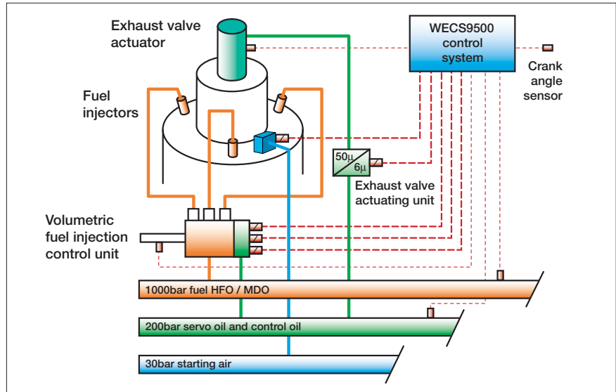
Fig. 15: Schematic of the common-rail system in Sulzer RT-flex engines. [02#007]
