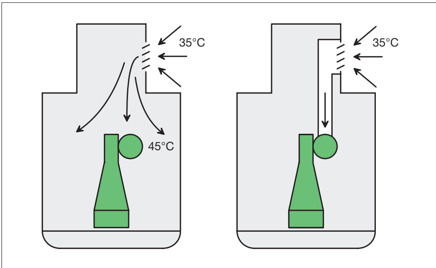
Fig. 2 Far left: Engine room air suction. Left: Ambient air suction. [04#038]
