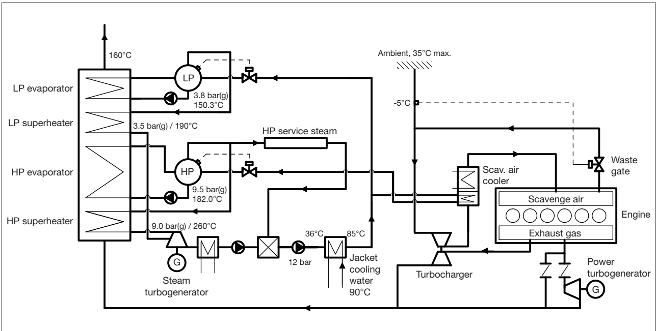
Fig. 9: Process diagram for the Total Heat Recovery Plant. [04#045]
