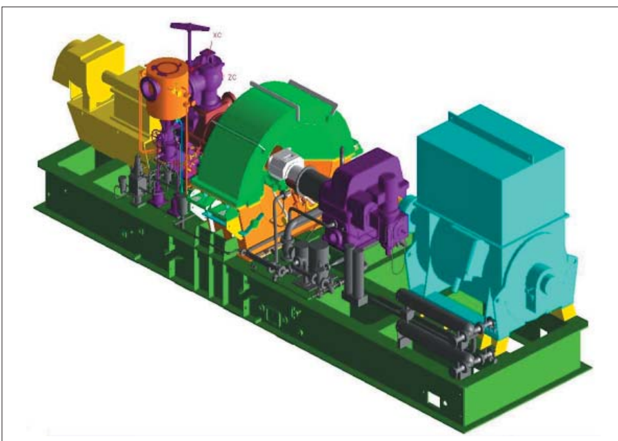
Fig. 6: Turbogenerator arrangement as proposed for about 7MWe output by Peter Brotherhood Ltd. The complete set measures about 9.5m long. [04#042]
