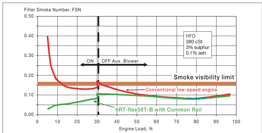
Fig. 16: Smoke measurements from the Sulzer 6RT-flex58T-B of the 'Gypsum Centennial' during sea trials, compared with an equivalent Sulzer RTA engine. According to a combinator characteristic. [02#010]
