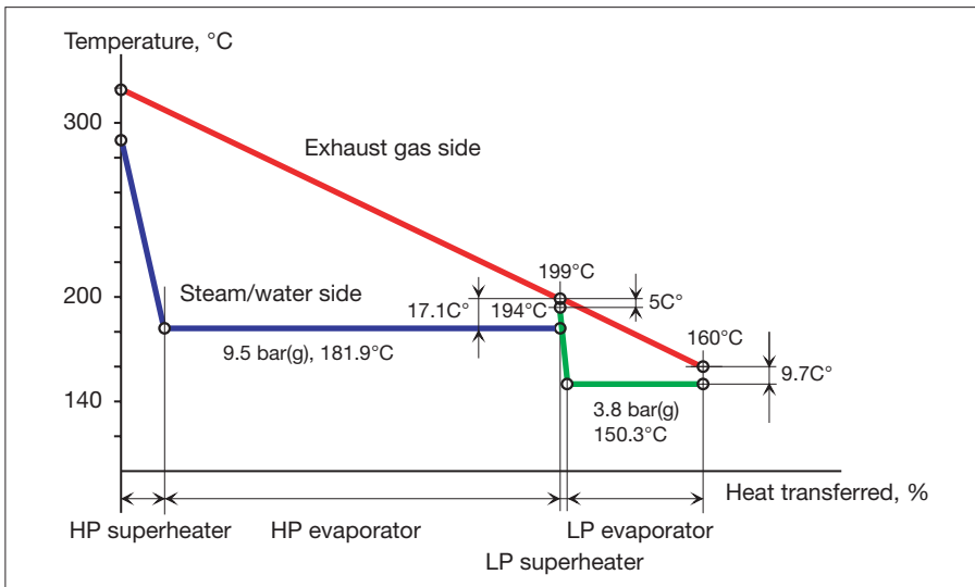
Fig. 5: Typical economiser diagram for the Total Heat Recovery Plant. [04#041]
