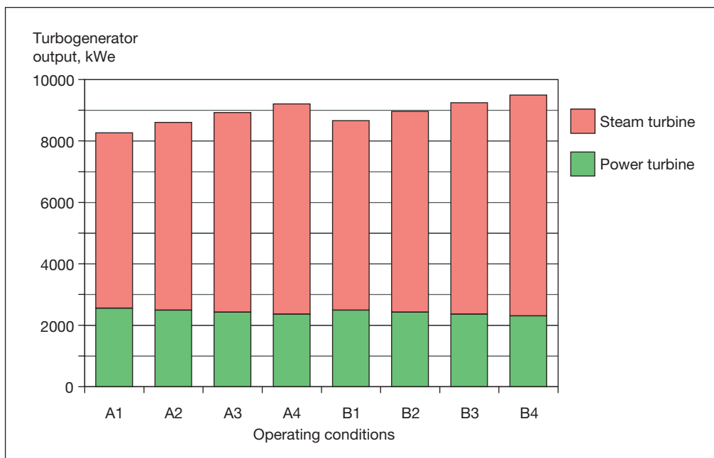
Fig. 10: Steam turbine and power turbine outputs at the various operating conditions, for the Sulzer 12RT-flex96C engine at 100% engine load. [04#046]
